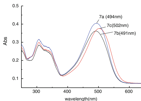
Fig. 3 UV-vis spectra of benzothiazole indole styryl cyanine dye bearing different substitutional groups on indole. ( c=7 \times 10^{-6} mol/L)
